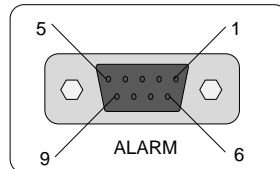
Figure 2: Contact closure alarm output connector
