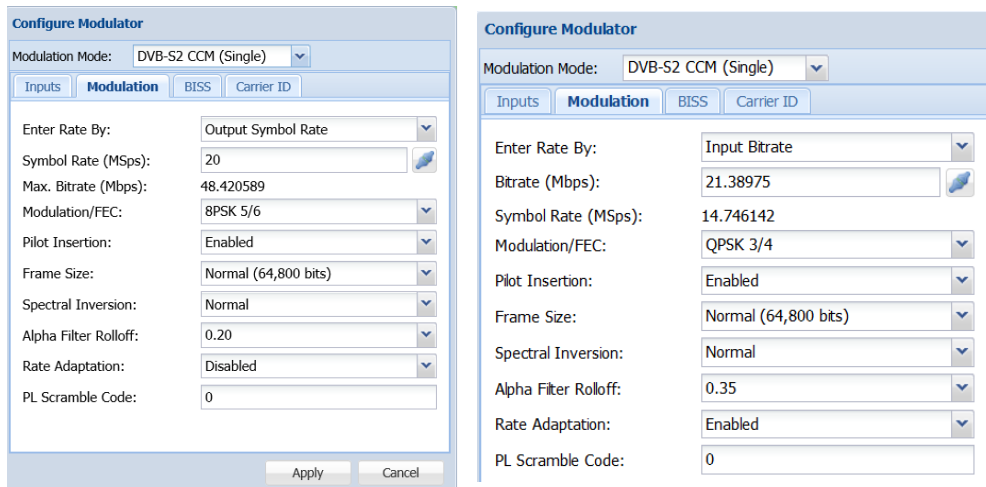
Figure 30: Single stream DVB-S2 Configuration
